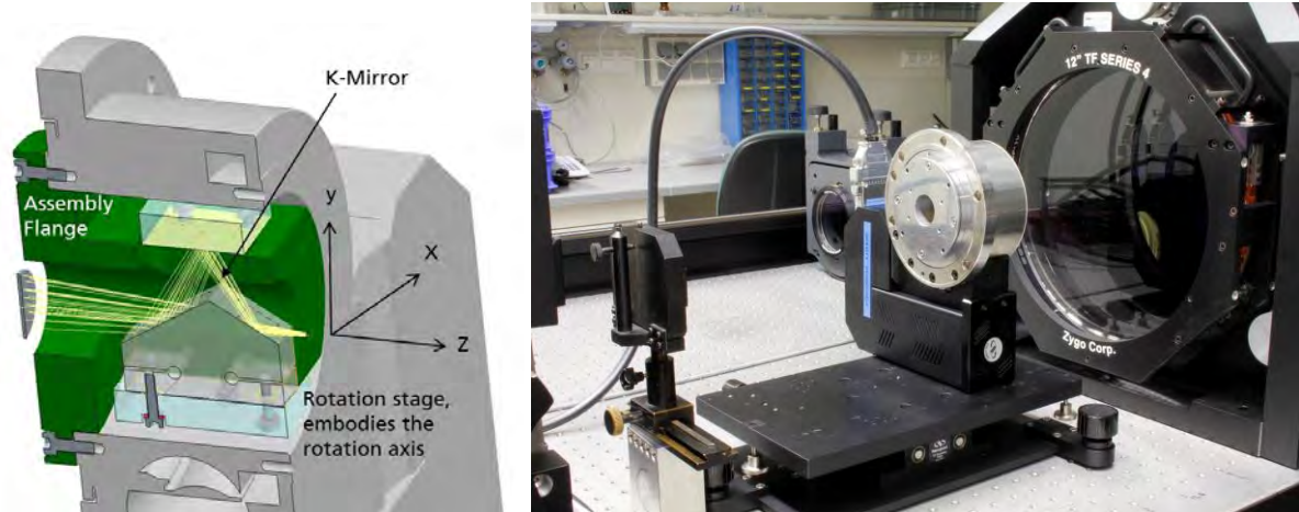
Fig. 6. Left: de-rotator with K-mirror assembly; Right: interferometric test setup for system alignment
