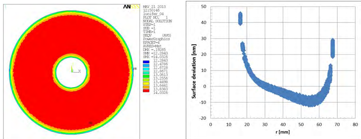
Fig. 4. Left: stress condition inside the NiP layer; Right: remaining form deformation (cross section) after removal of focus, z-shift, and intrinsic expansion of the mirror substrate.
