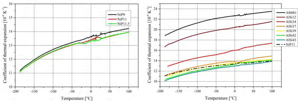
Fig. 2. Coefficient of thermal expansion for NiP layer with different phosphorous content (left) and for AlSi materials with different silicon content (right).
