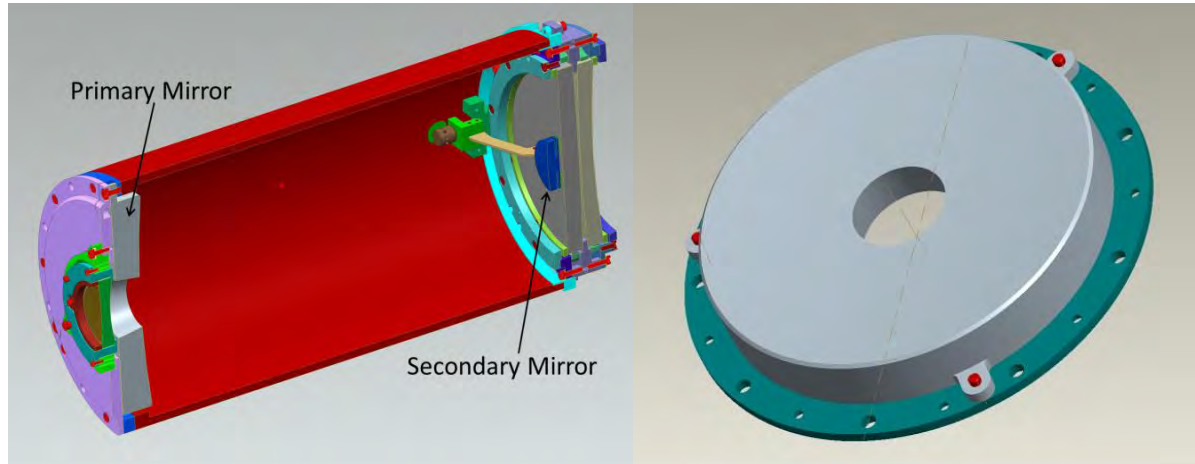
Fig. 3. Mechanical layout of the LUCI camera-optics (left) and of the primary mirror assembled on a mounting plate (right).
