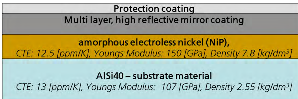
Fig. 1. Layout of a nickel plated AlSi40 mirror.
