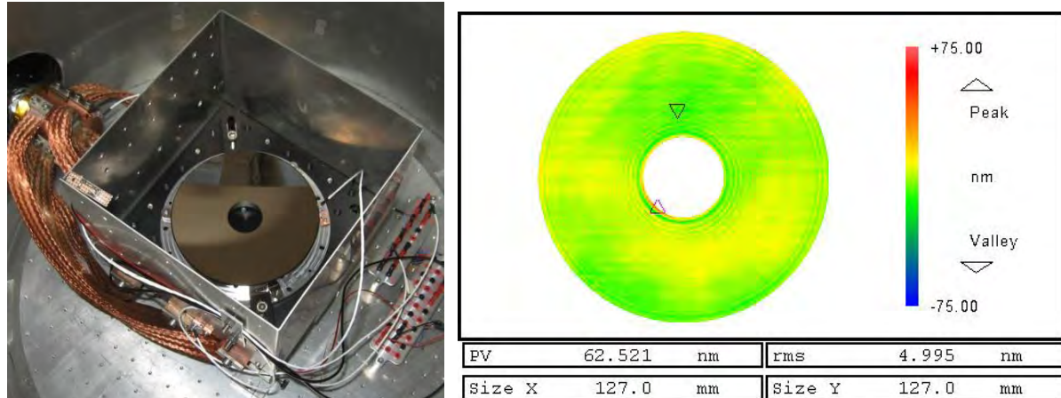
Fig. 5. Left: primary mirror mounted in the dewar for cryogenic characterization; Right: form deviation of the primary mirror after completion of all manufacturing steps @ ambient (22 °C) temperature.
